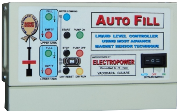
MAGNET SENSOR
